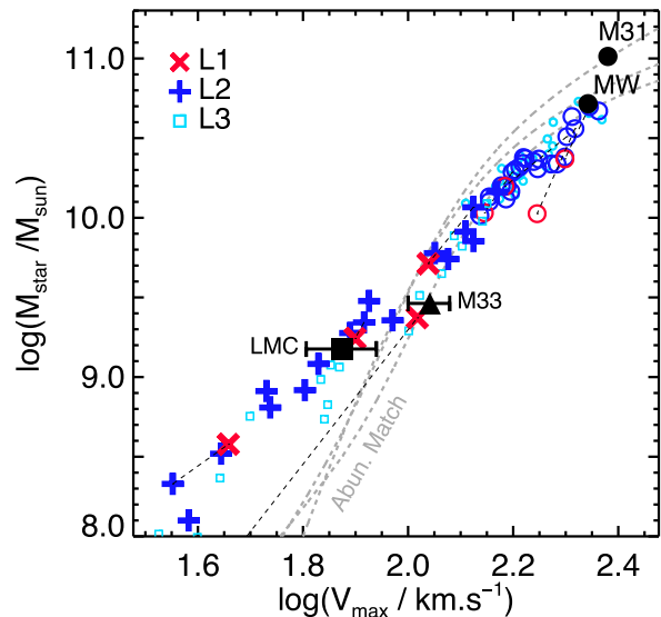
Figure 7. Stellar mass of the primary galaxies (circles) and their brightest satellites (crosses) for our 12 APOSTLE simulations, as a function of their maximum circular velocity. The large black solid symbols denote observational estimates for the two brightest members of the LG and their brightest satellites: MW, M31, LMC, and M33, respectively. Grey curves indicate ‘abundance matching’ predictions from Guo et al. (2010), Behroozi et al. (2013), and Kravtsov et al. (2014). Note that satellites as bright and massive as the LMC and M33 are not uncommon in our simulations. Note also that our primaries tend to be undermassive relative to observations and to predictions from abundance matching. The reverse applies at lower circular velocities. Black dashed lines connect matching systems at different resolution levels. See text for further discussion.
