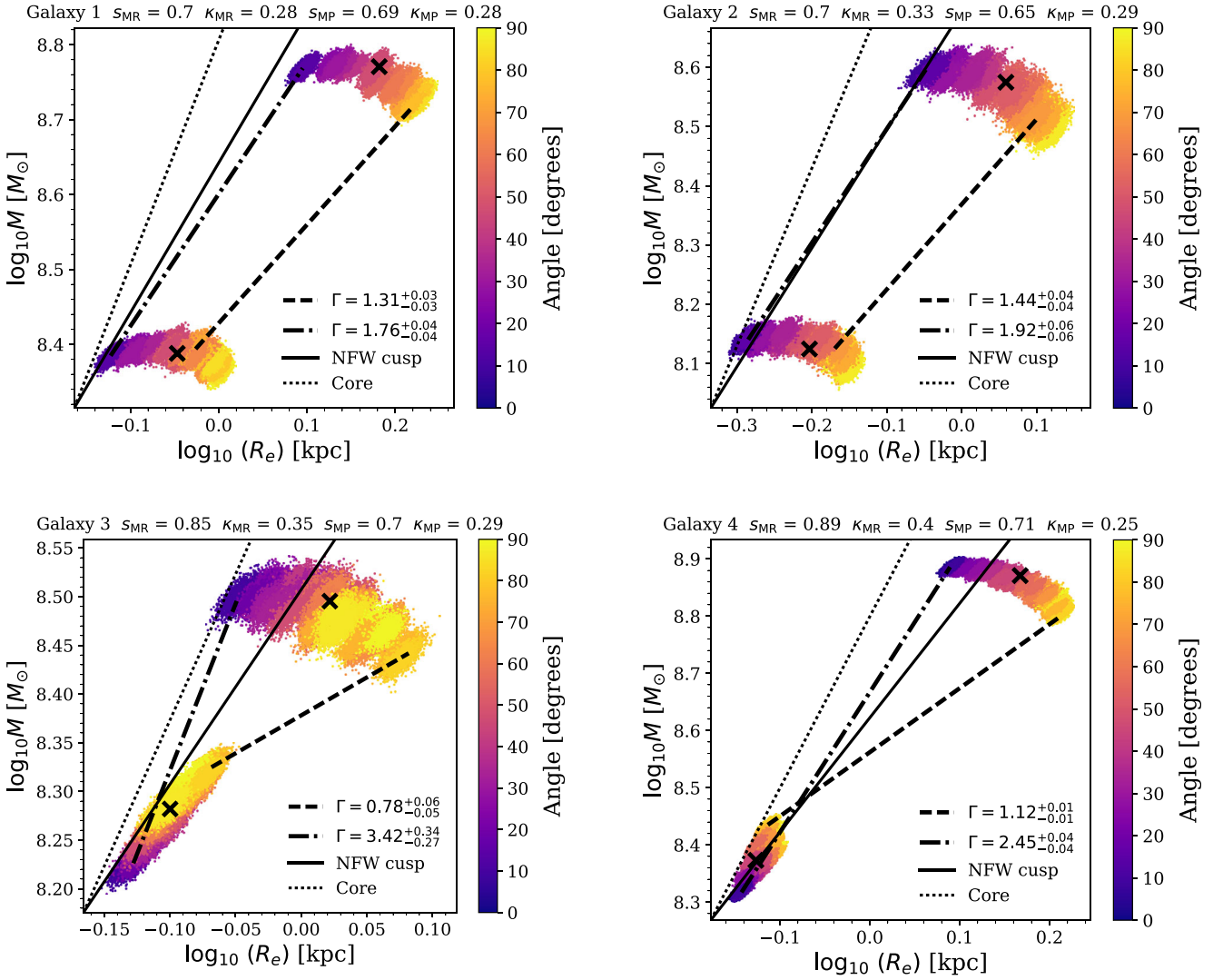
Figure 6. Logarithmic mass slopes for our four illustrative examples. The dots show measured projected half-mass radii and associated contained mass inferred from the Walker et al. (2009) estimator of equation (2) for each of the 1000 bootstrap resamplings of each galaxy; each galaxy is seen from 100 different directions. The points are coloured according to the viewing angle measured from the major axis of the metal-poor subpopulation. The black dashed and dash–dotted lines show the minimum and maximum slopes obtained from all 100 lines of sight, respectively. For reference, the black solid and dotted lines show the slopes of an NFW cusp and a core. The black crosses denote the true projected 3D half-mass radii and the masses within them, taken directly from the simulation. The labels above each panel give the sphericity and value of \kappa_{\text{rot}} for each subpopulation. A large scatter in projected half-mass radius can be seen in subpopulations that are strongly aspherical ( s < 1 ).
