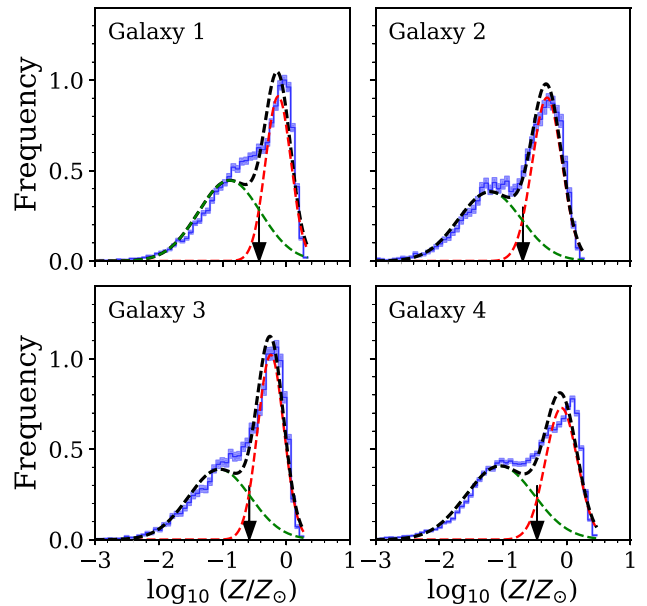
Figure 2. Metallicity histograms of the four galaxies that we use as case studies in this work. The blue curve represents the metallicity distribution and associated Poisson errors. The dashed black line shows the two-Gaussian fit. The dashed red and green lines show the individual Gaussians corresponding to the metal-rich and metal-poor subpopulations, respectively. The arrows show the metallicity at which the population is split. We have assumed a value of the solar metallicity of Z_{\odot} = 0.0127 .
