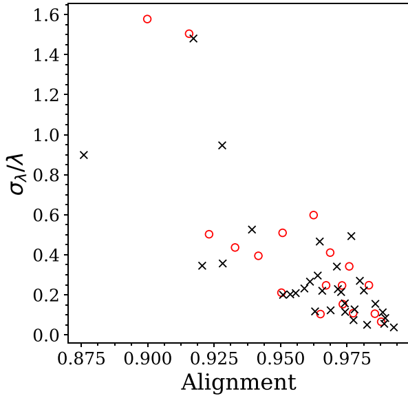
Figure 8. Relative upper error (the difference between the 84 th and the 50 th percentile divided by the median value) on the mass slope accuracy, \lambda , as a function of the alignment of the metal-rich and the metal-poor subpopulations, as defined in Section 3.1. Satellites and field galaxies are shown with red circles and black crosses, respectively. Measurements in galaxies with more misaligned subpopulations are more likely to return larger values of \Gamma .
