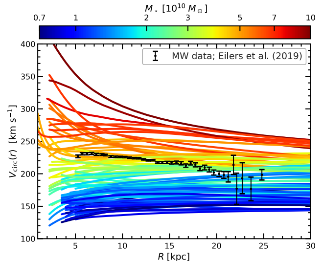
Figure 1. Rotation curves for the 87 simulated galaxies used in this work. Each line corresponds to one system. The lines are coloured according to the stellar mass of the galaxy (see legend at the top). The black symbols with error bars show the Eilers et al. (2019) determination of the MW rotation curve. The error bars correspond to the statistical uncertainties associated with the Eilers et al. measurement. For R > 20 kpc the MW measurement has large ( \sim 10 per cent or higher) systematic uncertainties and thus should be interpreted with care.
