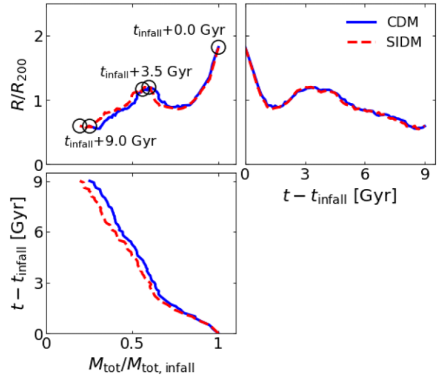
Figure 3. The median evolution since infall of cluster member galaxies with M_\star \gtrsim 10^7 M_\odot at z = 0 , in the CDM (solid blue) and SIDM (dashed red) versions of cluster CE-05. Top left-hand panel: cluster-centric distance in units of R_{200} versus galaxy mass in units of galaxy mass at infall. The labels indicate the time passed since infall, and the corresponding points on both tracks are encircled. Top right-hand panel: cluster-centric distance in units of R_{200} as a function of time since infall. Bottom left-hand panel: time since infall as a function of galaxy mass in units of the galaxy mass at infall. Note that a different number of galaxies contribute to the median at every point on the plot.
