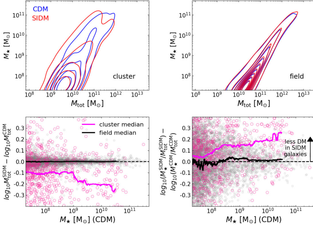
Figure 4. SHMR for galaxy pairs with >10 star particles ( M_{\star} \gtrsim 5 \times 10^7 M_{\odot} ), matched between CDM and SIDM simulations. Top panels: number-density contours of the stellar mass versus total mass in cluster CE-12 (left-hand panel) and the field (right-hand panel). Both are smoothed with the same circular Gaussian kernel of width \sigma = 0.35 dex: The increased scatter inside a cluster is real. A version for all (including unmatched) galaxies looks qualitatively similar. Bottom panels: the difference in total mass (left-hand panel) and stellar-to-halo mass (right-hand panel) between the SIDM and CDM galaxy populations. Pink points show matched galaxy pairs in cluster CE-12, with the running median overlaid; grey points show pairs in the field. The effect of SIDM is greatest for more massive galaxies.
