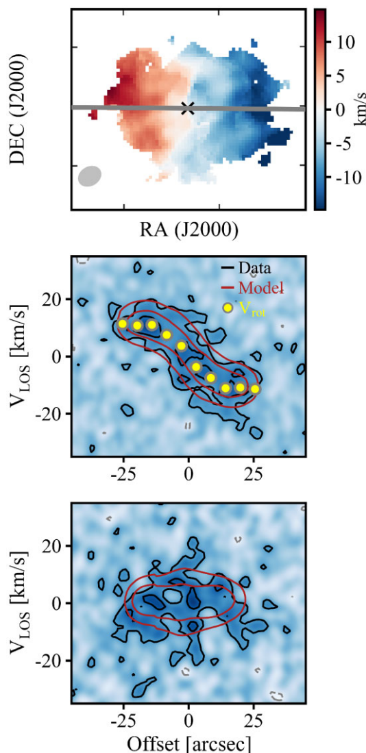
Figure 2. Top: Observed velocity field (same physical scale as the total HI map in Fig. 1); the grey ellipse shows the beam of the observations, the grey line the kinematic major axis, and the black cross the kinematic centre. Middle (Bottom): Major (minor)-axis PV diagram; data are shown in blue background and black contours (grey for negative values), and the best-fitting 3D Barolo azimuthal model in red contours. The yellow points show the recovered rotation velocities.
